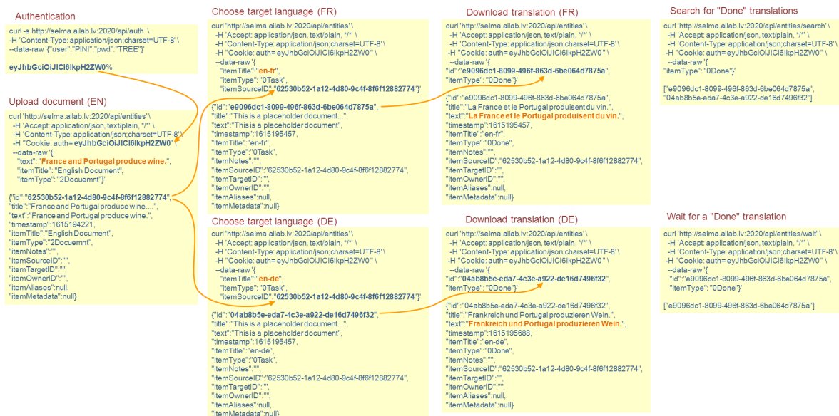
Figure 4 REST API access to PiniTree ontology editor database
