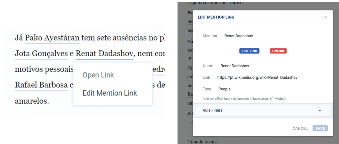
Figure 2 Feedback collection user interface for entity linking and NER
